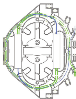
Splitter splice cassette with two assembled stainless tube 1:32 splitters - fiber guide
