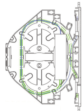
Splitter splice cassette fixed on base with assembled stainless tube 1:64 splitter - fiber guide
