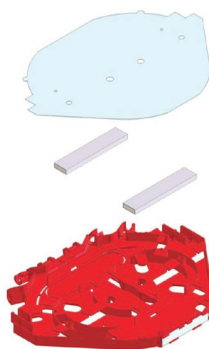
Splitter splice cassette with two assembled stainless tube 1:32 splitters
